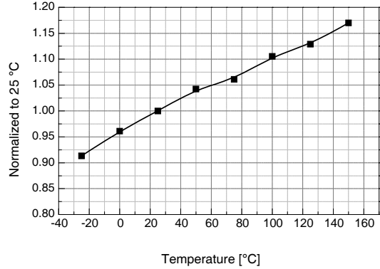
Figure 10. Feedback Sink Current vs. Temp.
