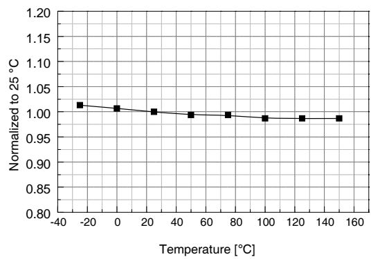
Figure 14. Over Voltage Protection vs. Temp.
